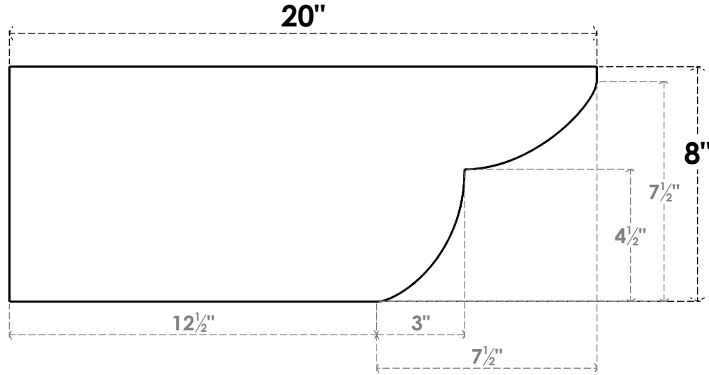
SIDE PROFILE
